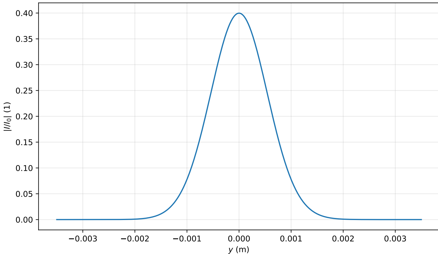
Intensity profile I(x=0, y, z=2.627)/I_0 , P_{in}=0.1P_{cr} , artificial time
